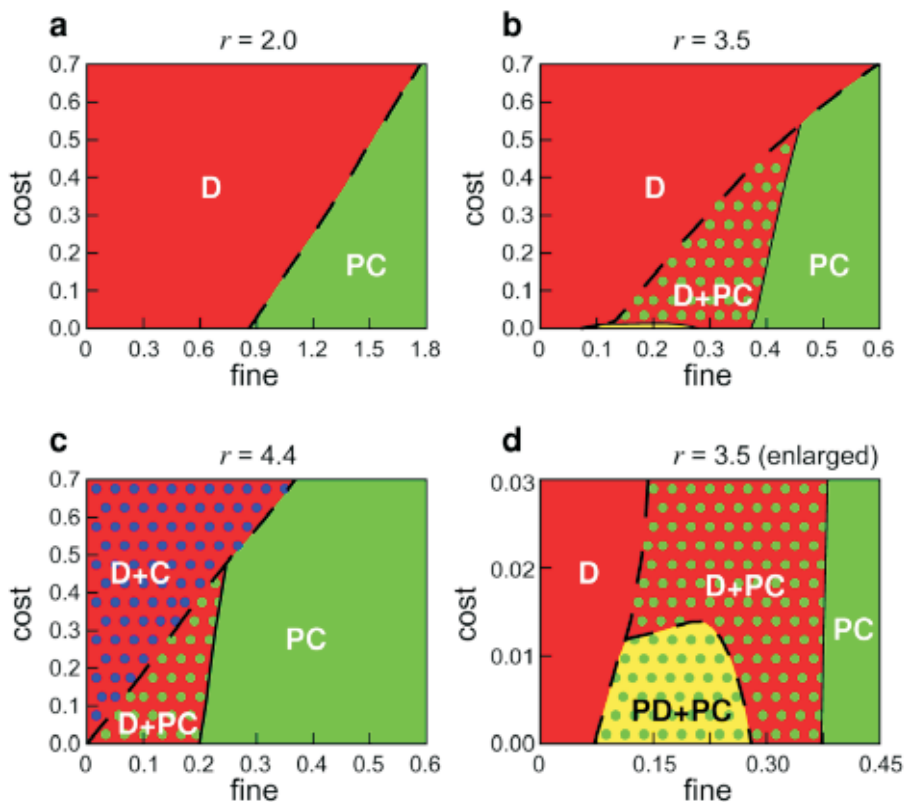
Figure 1. So-called “phase diagram”, showing the finally remaining strategies in the spatial public goods game with cooperators (C), defectors (D), cooperators who punish defectors (PC) and hypocritical punishers (PD), who punish other defectors while defecting themselves 39 . Initially, each of the four strategies occupies 25% of the sites of the two-dimensional lattice, in which individuals interact, and their distribution is uniform in space. However, due to their evolutionary competition, two or three strategies die out after some time. The finally resulting state depends on the punishment cost, the punishment fine, and the synergy r of cooperation (the factor by which cooperation increases the sum of investments). The displayed phase diagrams are for (a) r = 2.0 , (b) r = 3.5 , and (c) r = 4.4 . (d) Enlargement of the small- cost area for r = 3.5 . Solid separating lines indicate that the resulting fractions of all strategies change continuously with a modification of the punishment cost and punishment fine, while broken lines correspond to discontinuous changes. All diagrams show that cooperators and defectors cannot stop the spreading of costly punishment, if only the fine-to-cost ratio is large enough (see green PC area). Note that, in the absence of defectors, the spreading of punishing cooperators is extremely slow and follows a voter model kind of dynamics. A small level of strategy mutations (which continuously creates a small number of strategies of all kinds, in particular defectors) can largely accelerate the spreading of them. Furthermore, there are parameter regions where punishing cooperators can crowd out “second-order free-riders” (non-punishing cooperators) in the presence of defectors (D+PC). Finally, for low punishment costs, but moderate punishment fines, it may happen that “moralists”, who cooperate and punish non-cooperative behavior, can only survive through an “unholy alliance” with “immoral”, hypocritical punishers (PD+PC). For related videos, see http://www.soms.ethz.ch/research/secondorder-free-riders or http://www.matjazperc.com/games/moral.html .
